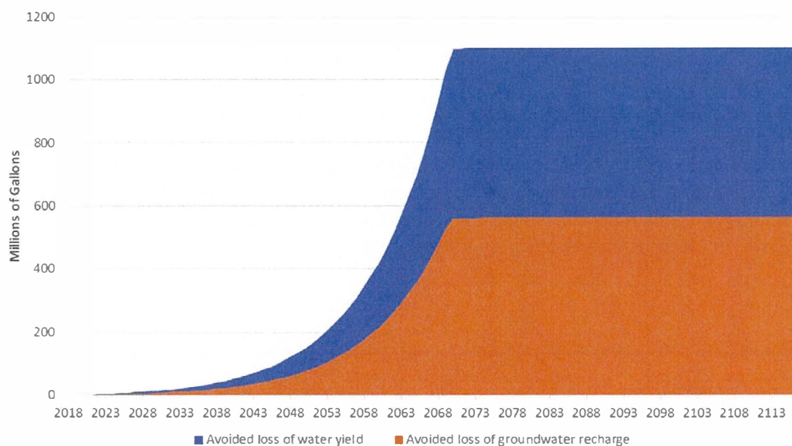
Figure 7. Avoided loss of freshwater yield and groundwater recharge as a result of conservation activities. 5
