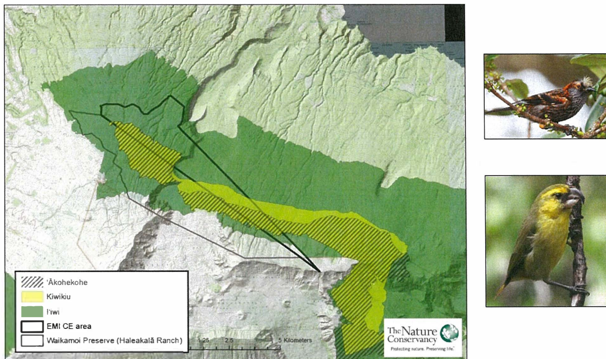
Figure 4. Endangered forest bird ranges in relation to EMI addition area. Updated bird ranges from Judge et al. 2
